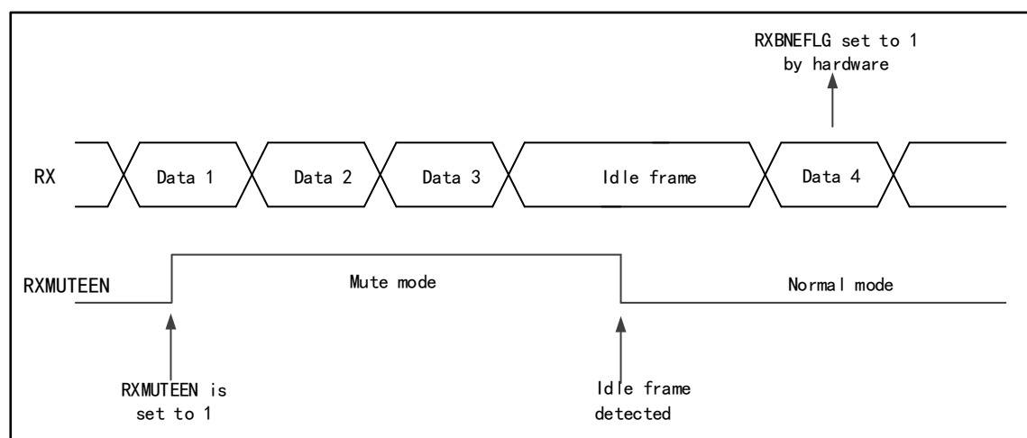
Figure 63 Idle Bus Exit Mute Mode
