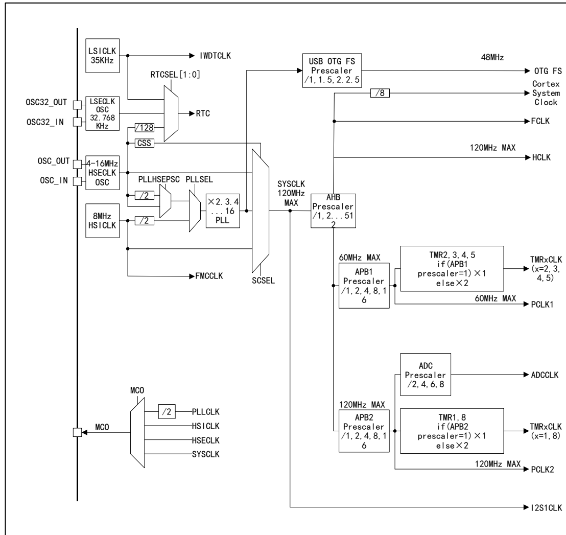
Figure 4 APM32F403xB Clock Tree
