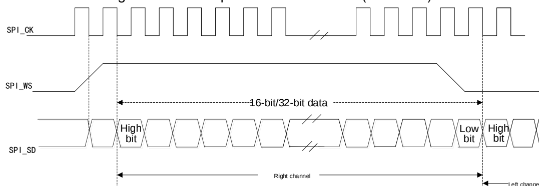
Figure 86 I2S Philips Protocol Waveform (16/32 bits)
