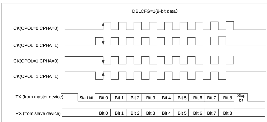
Figure 67 USART Synchronous Transmission Timing Diagram (DBLCFG=1)
