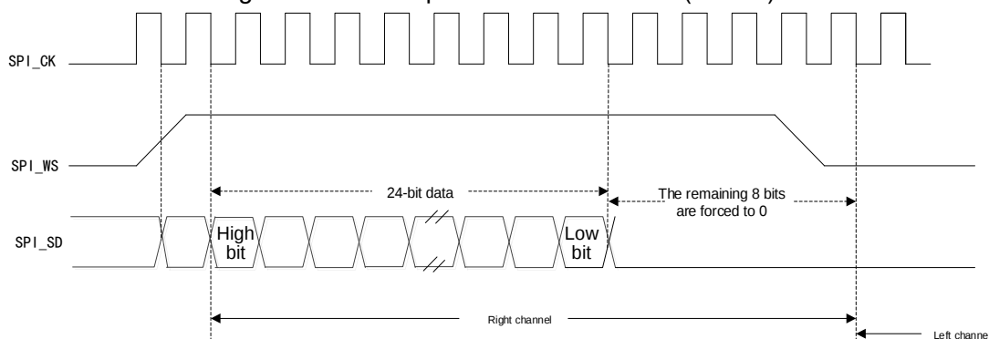
Figure 87 I2S Philips Protocol Waveform (24 bits)
