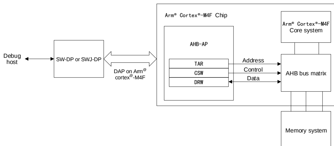
Figure 15 APM32F403xB Level and Arm® Cortex®-M4F Level Debugging Block Diagram
