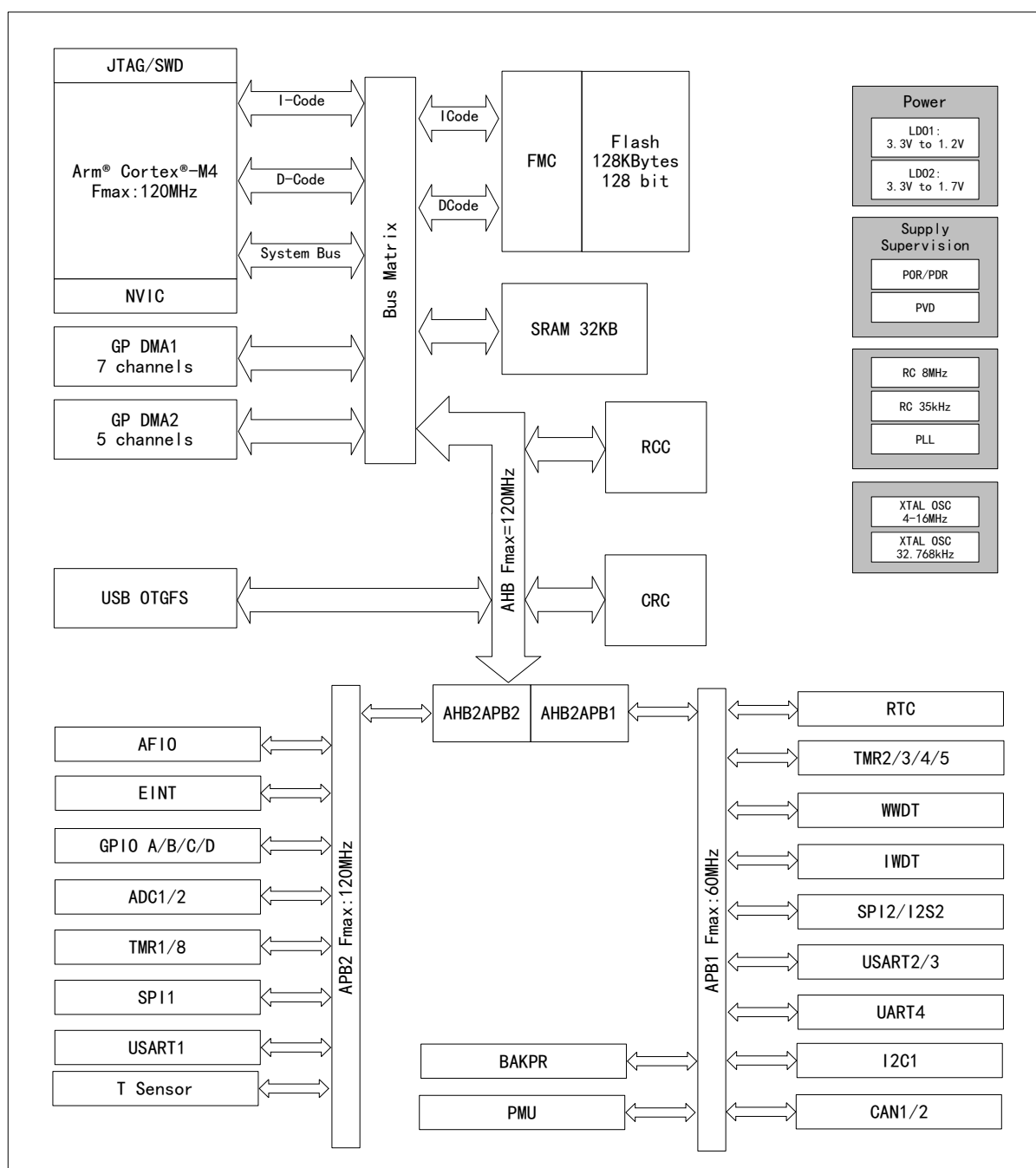
Figure 1 APM32F403xB System Architecture Block Diagram
