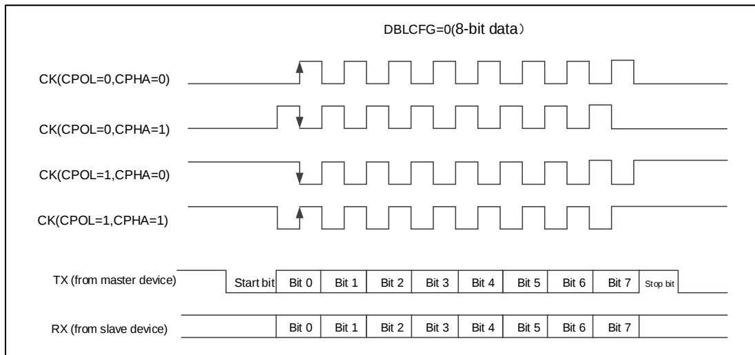
Figure 66 USART Synchronous Transmission Timing Diagram (DBLCFG=0)
