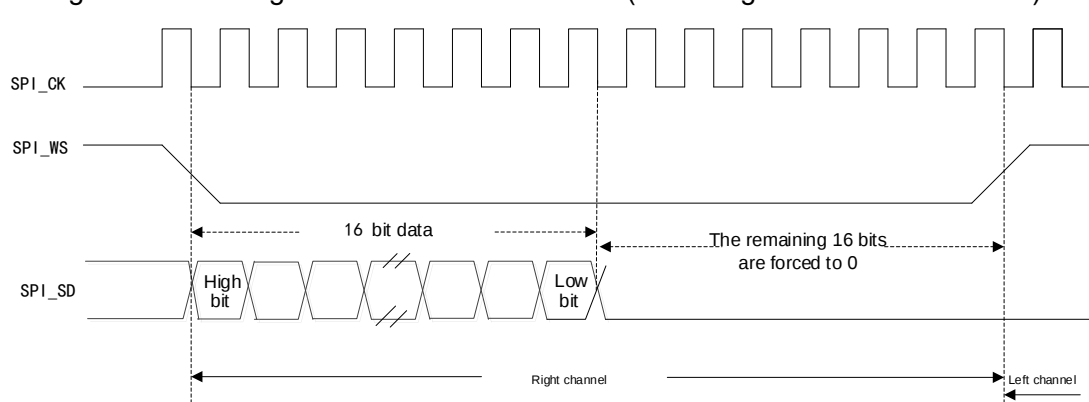
Figure 91 MSB Alignment Standard Waveform (extending from 16 bits to 32 bits)
